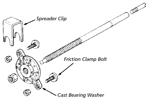
She-Bolt with Cast Bearing Washer
