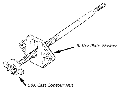
She-Bolt with Batter Plate Washer
