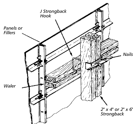
Strongback Attachment
