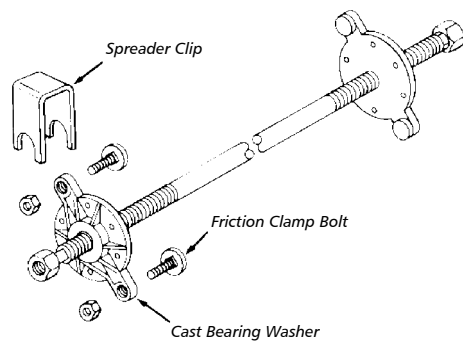
Taper Tie with Cast Bearing Washer
