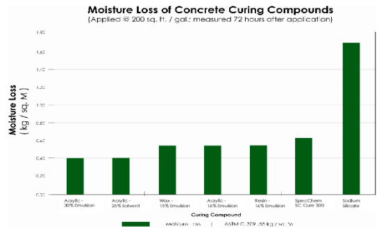
Moisture Retention Comparison Chart for Concrete Curing Compounds for Hard Trowel Finish
